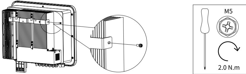
Fig. 2.3 Wall mounted bracket
