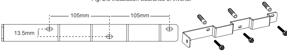
Fig. 2.1 Inverter rack
