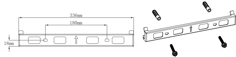
Fig. 2.1 Wall-mounting bracket
