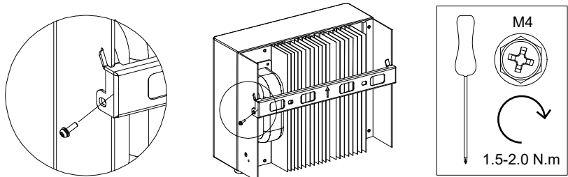
Fig. 2.3 Wall mounted bracket
