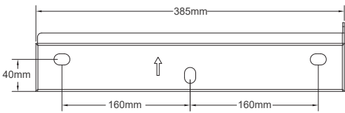
Fig. 2.1 Inverter rack
