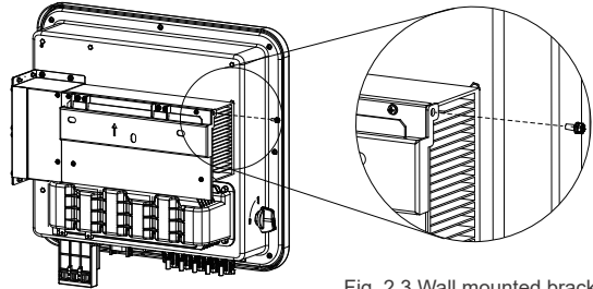
Fig. 2.3 Wall mounted bracket
