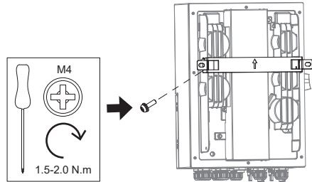
Fig. 2.3 Wall mounted inverter
