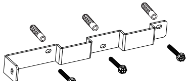
Fig. 2.2 Wall mounted bracket
