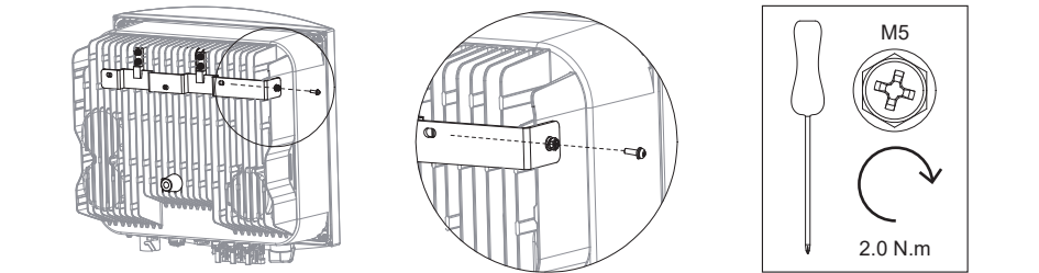
Fig. 2.3 Wall mounted inverter
